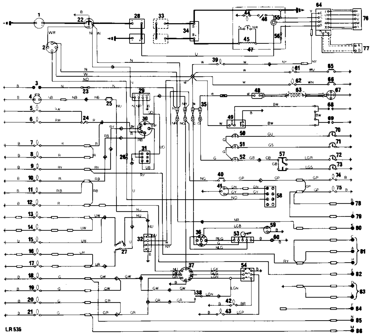
Fig. 149 Circuit diagram. 24 volt models. Transistored charging system.
