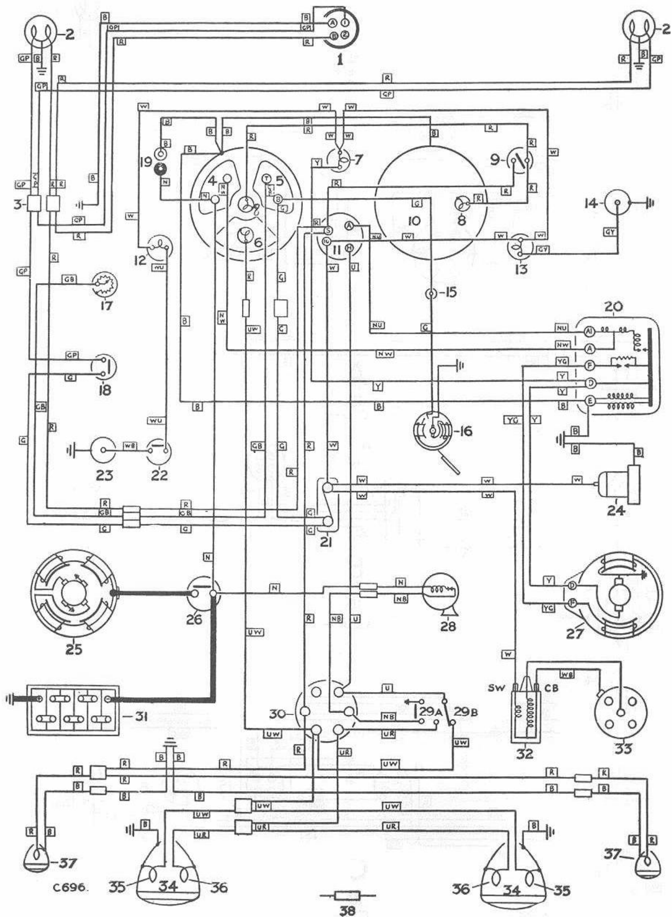
Fig. P-8—Wiring diagram 88 and 109—1954-58 models
