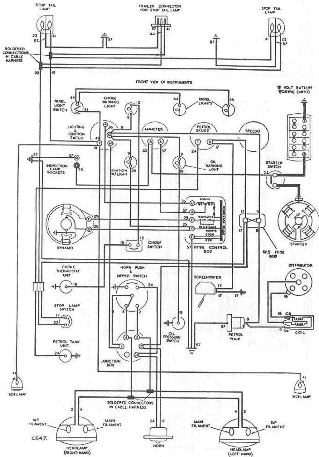
Fig. P-3—Wiring diagram, 1948-50 models
